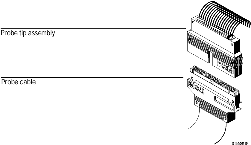
Connecting Probe Tip Assembly
